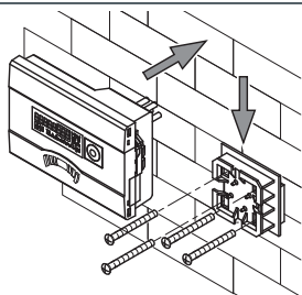
Wall mounting
