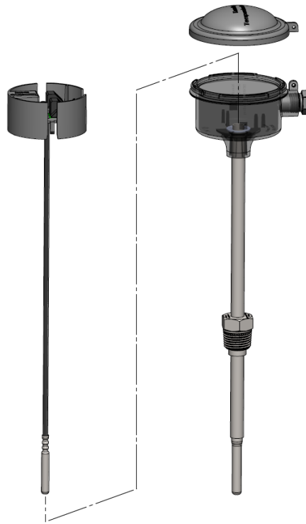
Figure 13: A \varnothing 5.8 mm pocket sensor with connection head can, for example, be mounted in a tee as shown in Figure 14.
