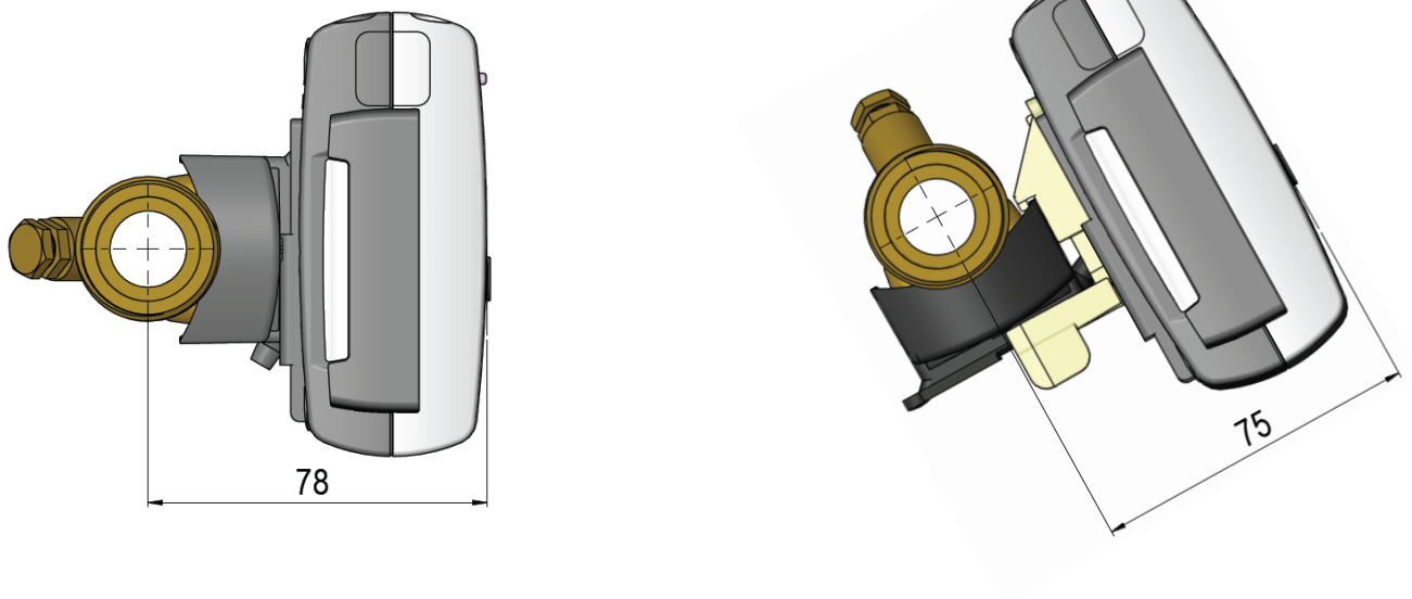
Figure 5: MULTICAL® 603 mounted on ULTRAFLOW® with G \frac{3}{4} threaded connection
