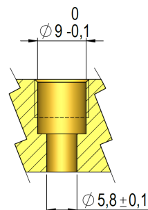
Figure 11: Measurement and tolerance requirements when installing a direct \varnothing 5.0 mm or \varnothing 5.2 mm temperature sensor.
