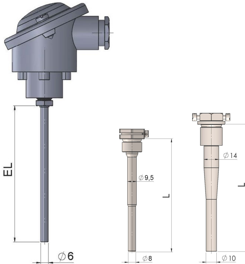
Figure 15: ø6 mm pocket sensor with connection head and matching pockets.
