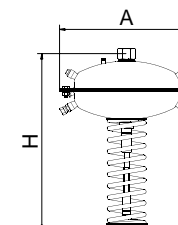
AFQ2 (28 kg)
