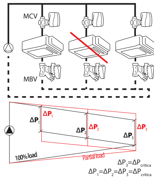
Fig 11.2 Partial load - reverse return system
