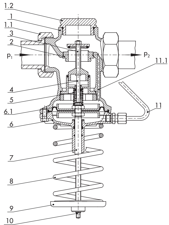
Fig. 3: Type 45-6, DN 15 to 50 · With connection nuts and welding ends
