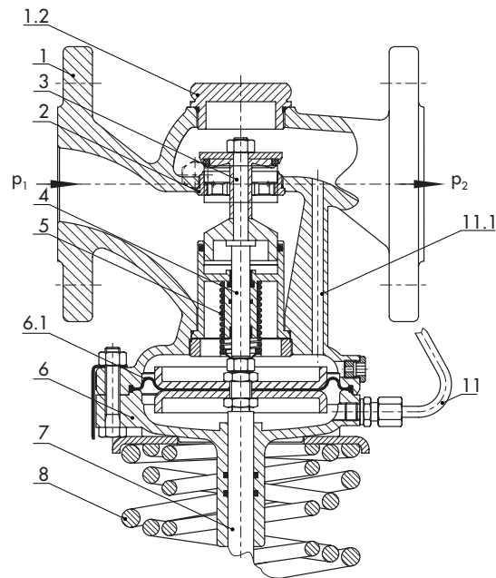
Fig. 4: Type 45-6, DN 32 to 50 · With flanged body valve
