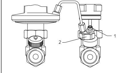
Illustr. 6.1: "Hycocoen DTZ", capillary connection, installation
