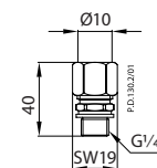
Compression fitting
