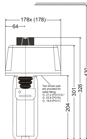
Fig. 3. ML6421B / ML7421B (dimensions in mm)
