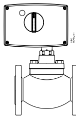
VB2 20, 30; VB2 23, 33 VB2 DN 15 - 50
