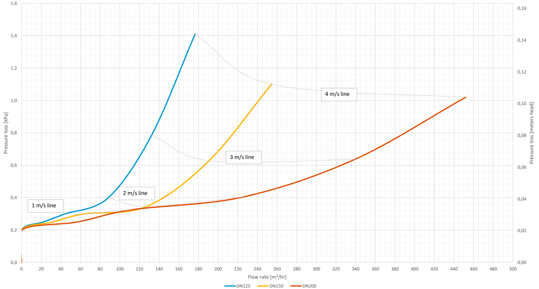
Pressure loss - Series 41 - Bare Shaft - DN125, DN150 and DN200
