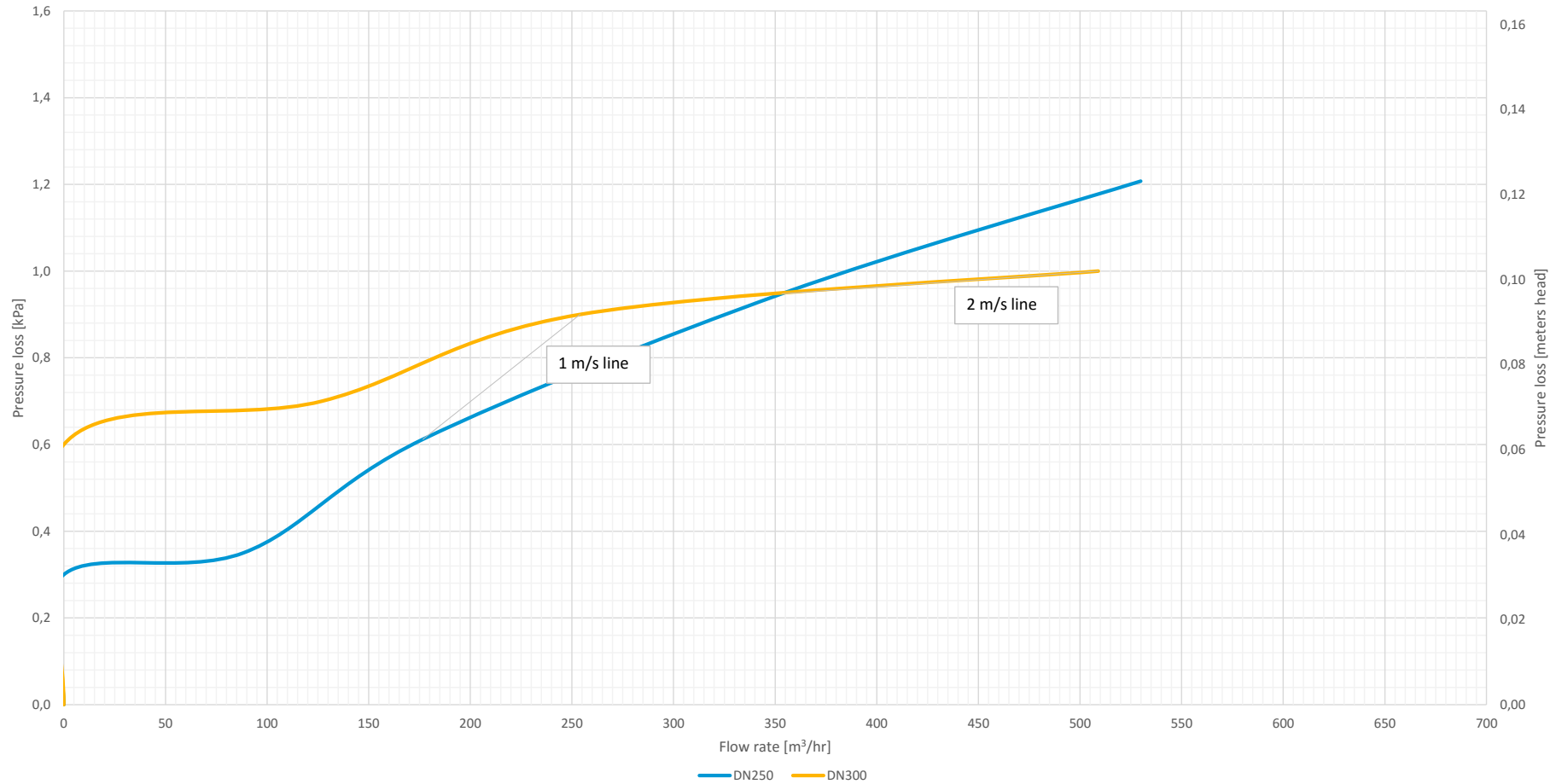
Pressure loss - Series 41 - Bare Shaft - DN250 and DN300
