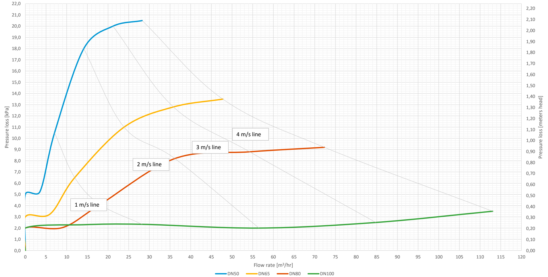
Pressure loss - Series 41 - Spring - DN50, DN65, DN80 and DN100
