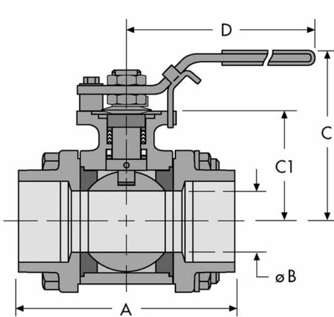
1/2" - 2 1/2" VALVES
