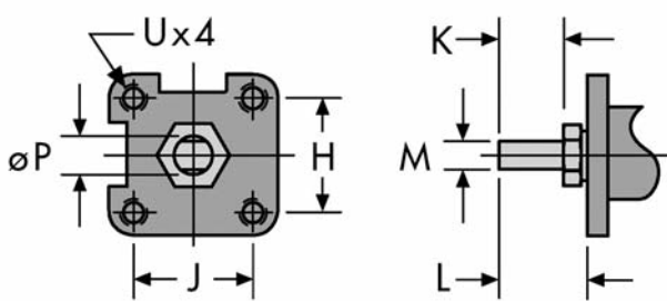
1/4" - 2 1/2" VALVES
