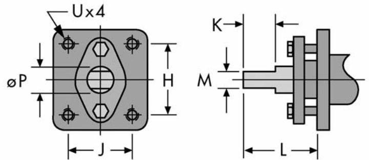
3"-12" VALVES
