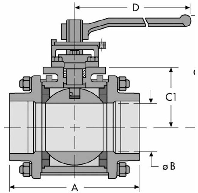
3"-12" VALVES
