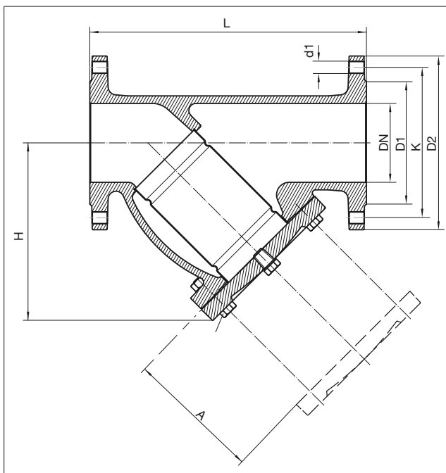
Illust. 2: Dimensions
