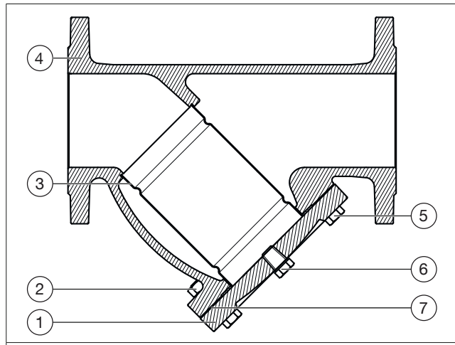
Illust. 1: Construction of the strainer
