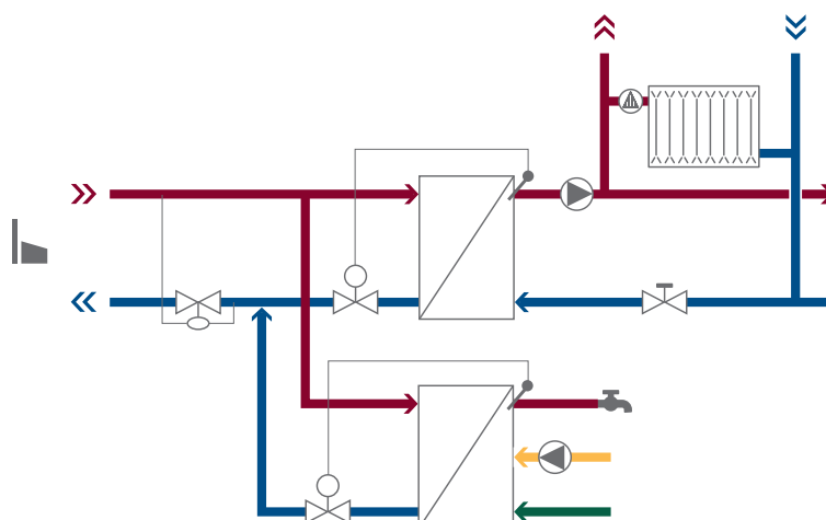
Example of self-acting controlling
